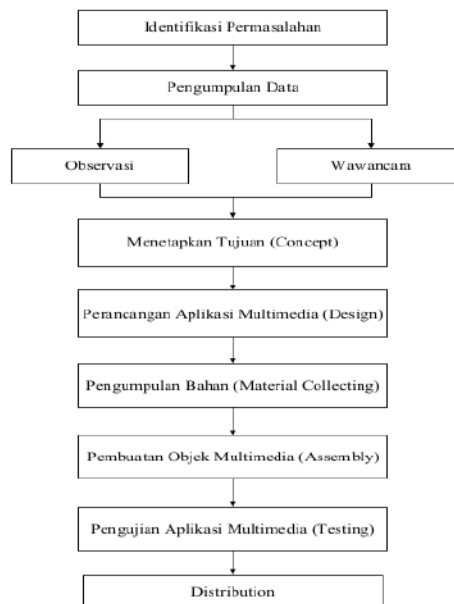
Gambar 1 Diagram Alur Langkah-langkah Penelitian
