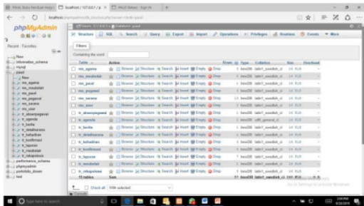
Fig. 22. Database implementation.
