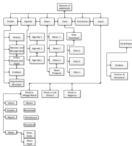
Fig. 15. Navigation structure.
